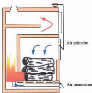
COMBUSTION HORIZONTALE
